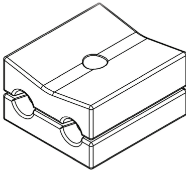
AGC Series ADSS Download Clamp with galvanized steel hardware
