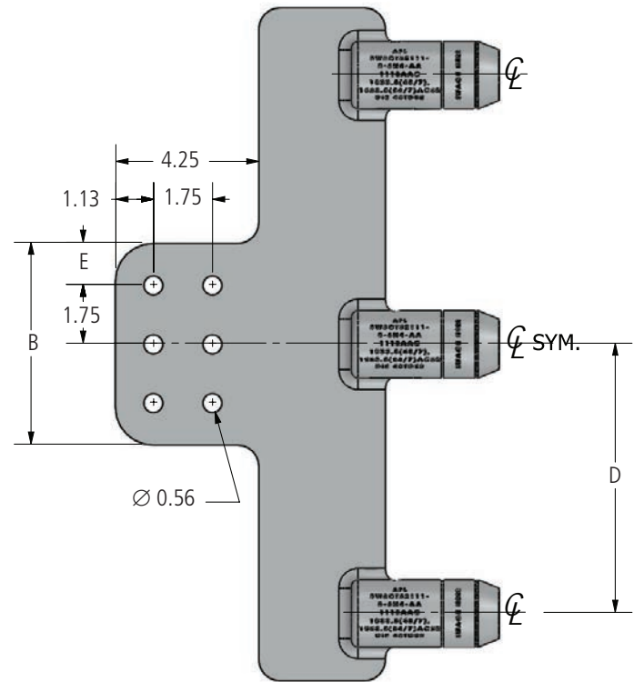
Pad Detail 2
