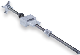
Removal Tool for OPGW Wedge Dead End
