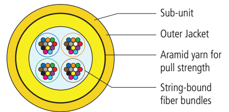
Ruggedized 48 fiber
