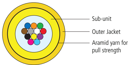
Ruggedized 12 fiber
