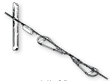
In-Line Splice
